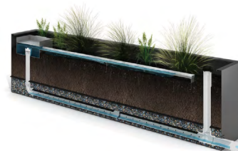
Water enters perforated drainpipe and exits.
