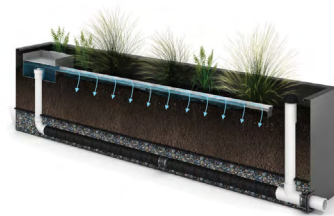
Water trickles through perforations into media.
