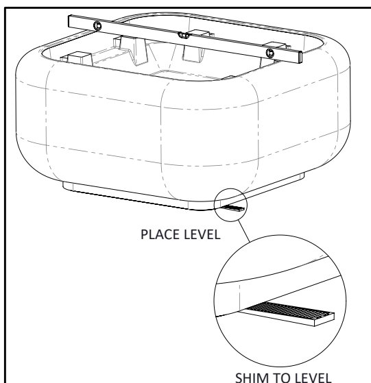
Leveling basin of single water feature.
