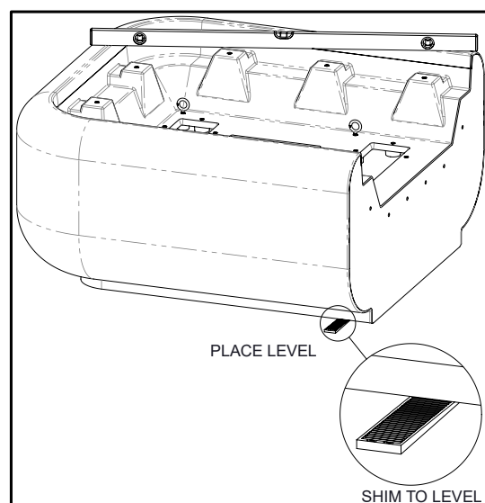
Leveling of start/end basin of double & triple water feature.
