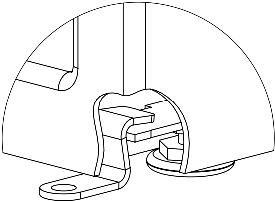
OPTIONAL, ANCHORING KIT (WT-AKIT) INSTALLED IN FIELD 3/8" ANCHORS (NOT INCLUDED)
