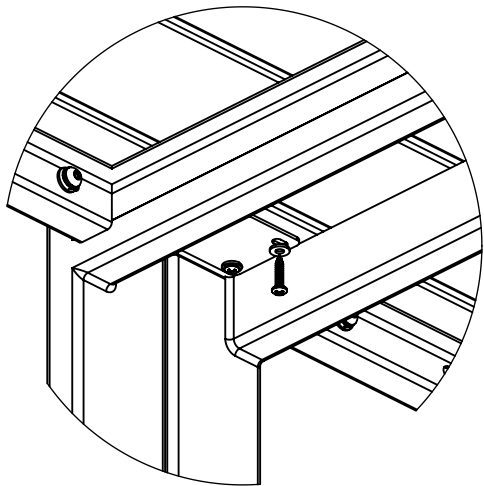
OPTIONAL, BENCH JOINING KIT (WT-JKIT) INSTALLED IN FIELD WITH HARDWARE PROVIDED SCALE 1 : 6
